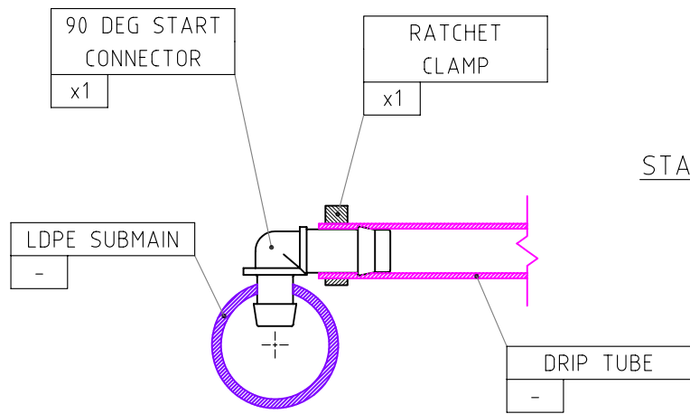
90 DEG START CONNECTOR
