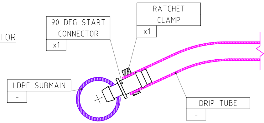
STANDARD START CONNECTOR
