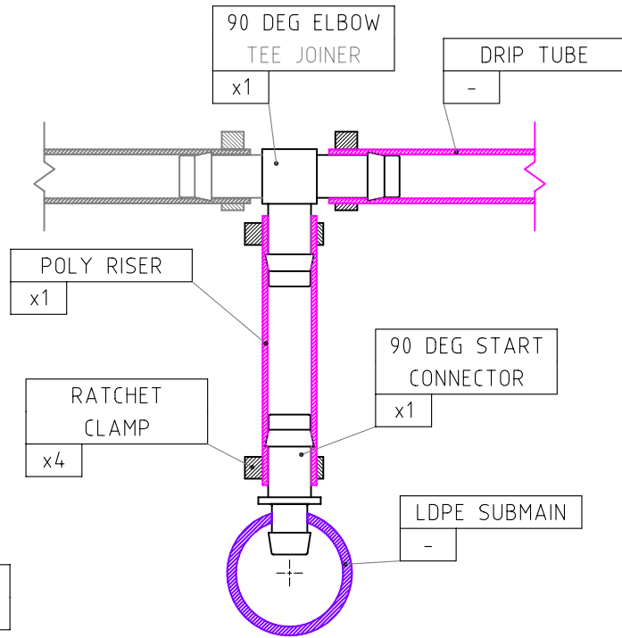
STANDARD START CONNECTOR WITH RISER
